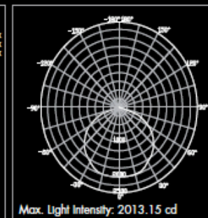
Candle Power Distribution
