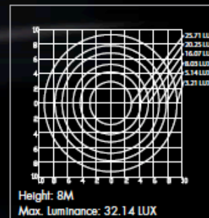
ISO-Luminance Curve
