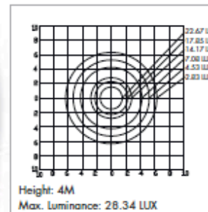
ISO-Luminance Curve
