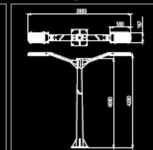
Dimensions of System
