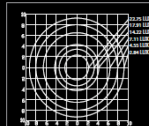
Light Sensor
