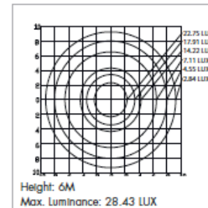
ISO-Luminance Curve
